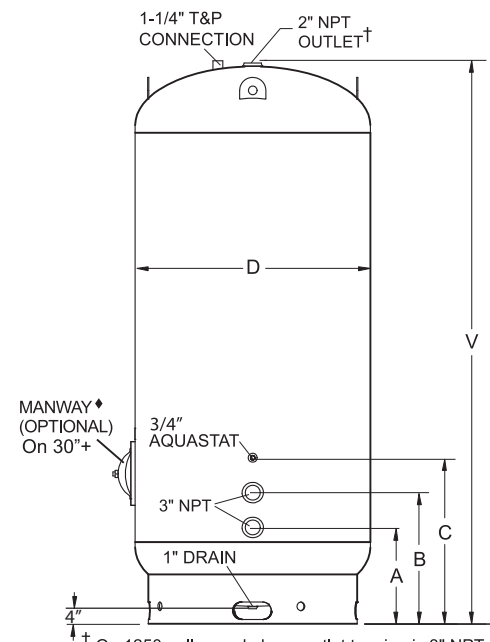
30" DIAMETER AND LARGER TANKS
