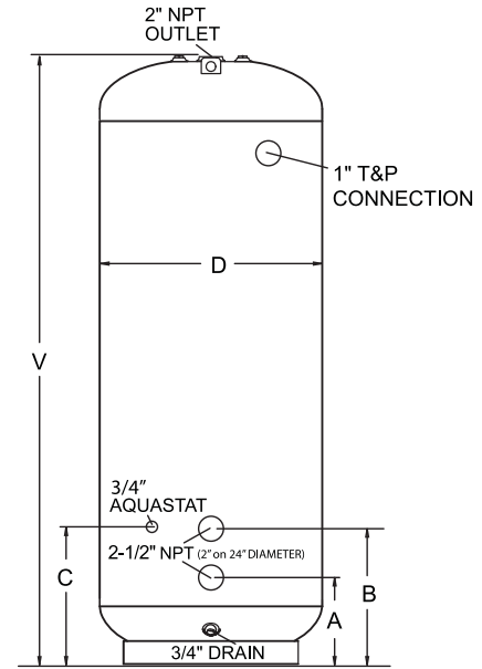
24" & 28" DIAMETER TANKS
